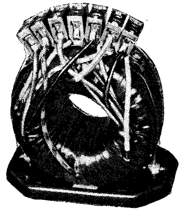
A ring-type core and toroidal windings are used in the Erka mains transformer.
