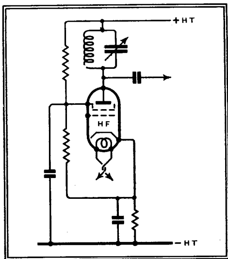
Fig. 2.—A common example of a feed system to a screen grid or pentode valve in which adjustment of screen voltage would influence grid bias also.
