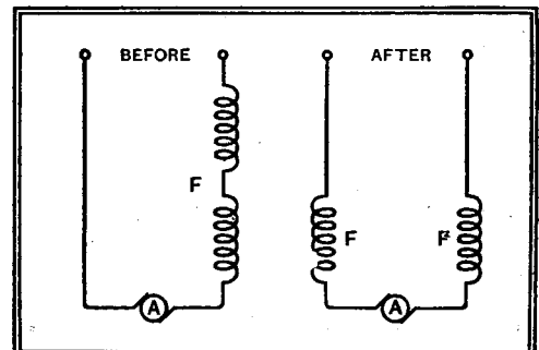
Re-arrangement of field coils FF to minimise radiation of interference produced at the commutation A.
