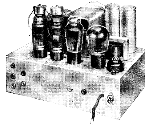
The "all-pentode" HF-det.-LF model, like its companion 2-valve set, covers short waves between 20 and 60 metres as well as the normal broadcast bands.
