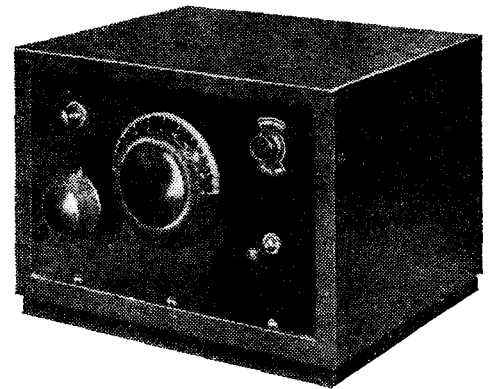
The National Radio Service Company's crystal set, designed by Mr. R. W. Hallows to cope with modern conditions. A wave-trap for eliminating local-station interference is included.
