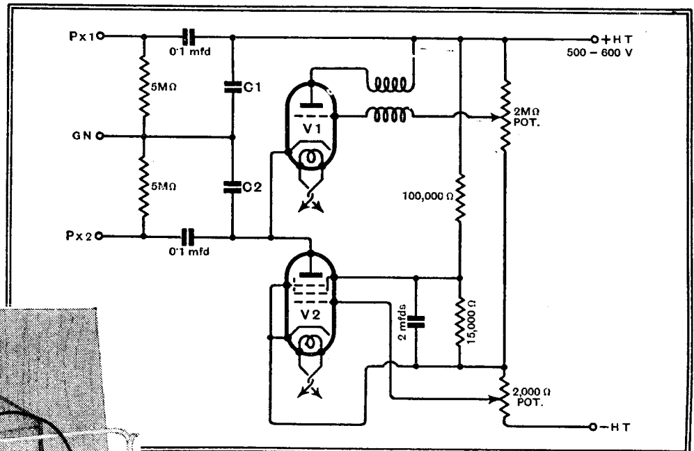
The screen-grid valve in the above circuit performs the function of a saturated diode, and the triode acts to discharge the condensers C_1 and C_2 at the end of the stroke. An experimental time base built for a low-frequency is shown at the left.
