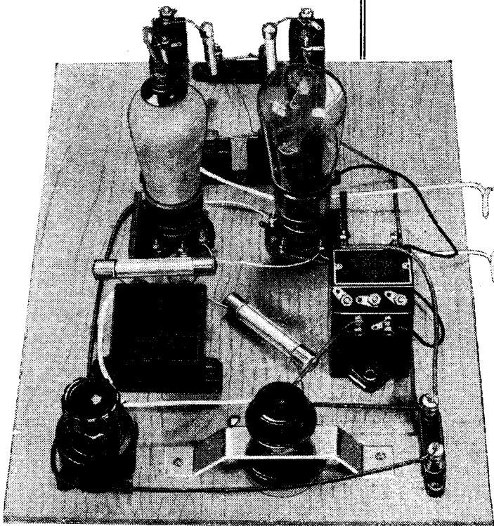
The screen-grid valve in the above circuit performs the function of a saturated diode, and the triode acts to discharge the condensers C_1 and C_2 at the end of the stroke. An experimental time base built for a low-frequency is shown at the left.
