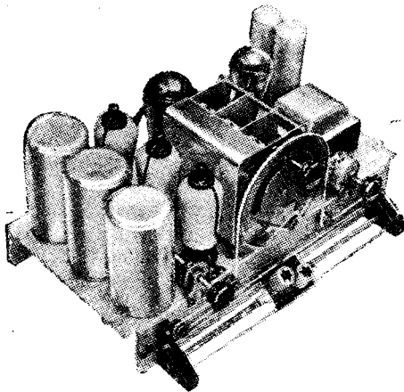
The chassis of the Ultra Panther receiver: a straight set with two HF stages and three tuned circuits.
