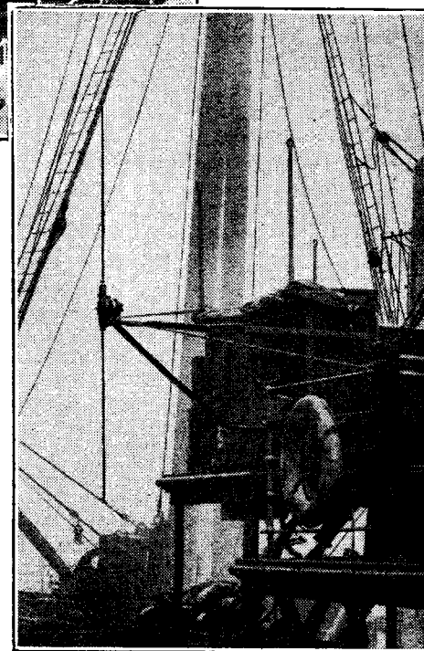
Beam receiving antenna on S.S. "Royal Scot."
