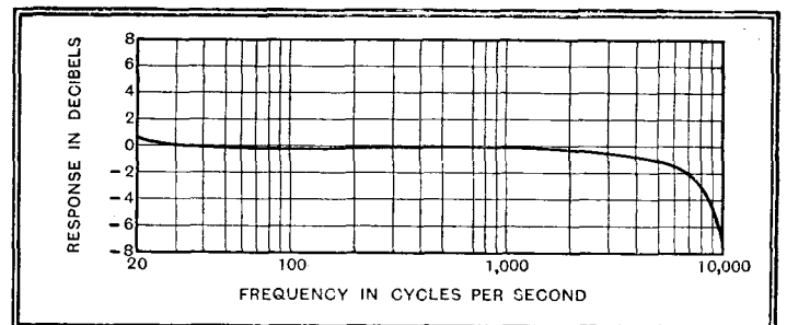
The overall frequency response curve of the Ferranti AC12C amplifier includes the losses in the output transformer.
